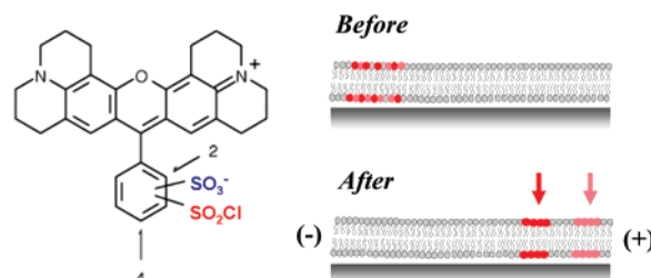
Figure 2. Left: Chemical structure of Texas Red sulfonyl chloride. 22 The lower ring contains the reactive sulfonyl chloride group (red), which can reside at either the 2 (ortho) or 4 (para) position. Right: Illustration of the separation of a mixture of Texas Red DHPE lipid isomers into distinct bands in a supported bilayer.
