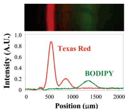
Figure 4. Top: Composite image of the separation of Texas Red DHPE and BODIPY DHPE in a POPC bilayer containing 25 mol % of cholesterol after 35 min of applying a 100 V potential. Bottom: Corresponding linescan of the image, corrected for vignetting. The small peak at \sim 300 \mu\text{m} represents an approximately 2% immobile fraction of total dye-labeled molecules. The areas of the large and small peaks of Texas Red are \sim 75 to 25%, which is slightly different than the areas in Figure 1 and probably represents a small amount of batch-to-batch variability in the dye formulation of the manufacturer.
