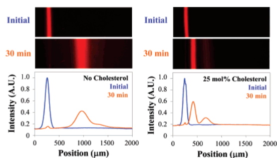
Figure 1. Comparison of the band broadening of Texas Red labeled lipids migrating in either pure POPC (left) or POPC doped with 25 mol % of cholesterol (right). The upper two images are epifluorescence micrographs of the systems immediately after formation of the Texas Red containing strips. The lower two images show band migration after applying 100 V across the sample for 30 min. The positive and negative electrodes were located on the right and left sides of the frame, respectively. The faint line to the left in the bottom panels represents a 2% immobile fraction of lipids. The plots below the images show the corresponding linescans initially and after 30 min. The linescans have been corrected for vignetting and normalized to the fluorescence level of the initial image to account for photobleaching. The length of the images matches the scale of the x-axis in the plots.
