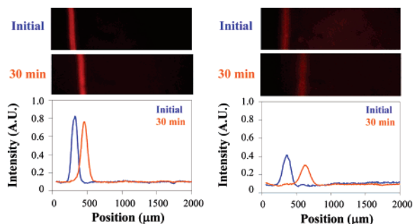
Figure 3. Images of Texas Red DHPE migrating through a 75 mol % of POPC/25 mol % of cholesterol bilayer after TLC purification. Left: Texas Red from the large mol fraction isomer after TLC purification, initially (top) and after 30 min of 100 V applied potential (middle). Right: Corresponding images for the other isomer. The plots below the images show the associated linescans, initially and after 30 min, corrected for vignetting.
